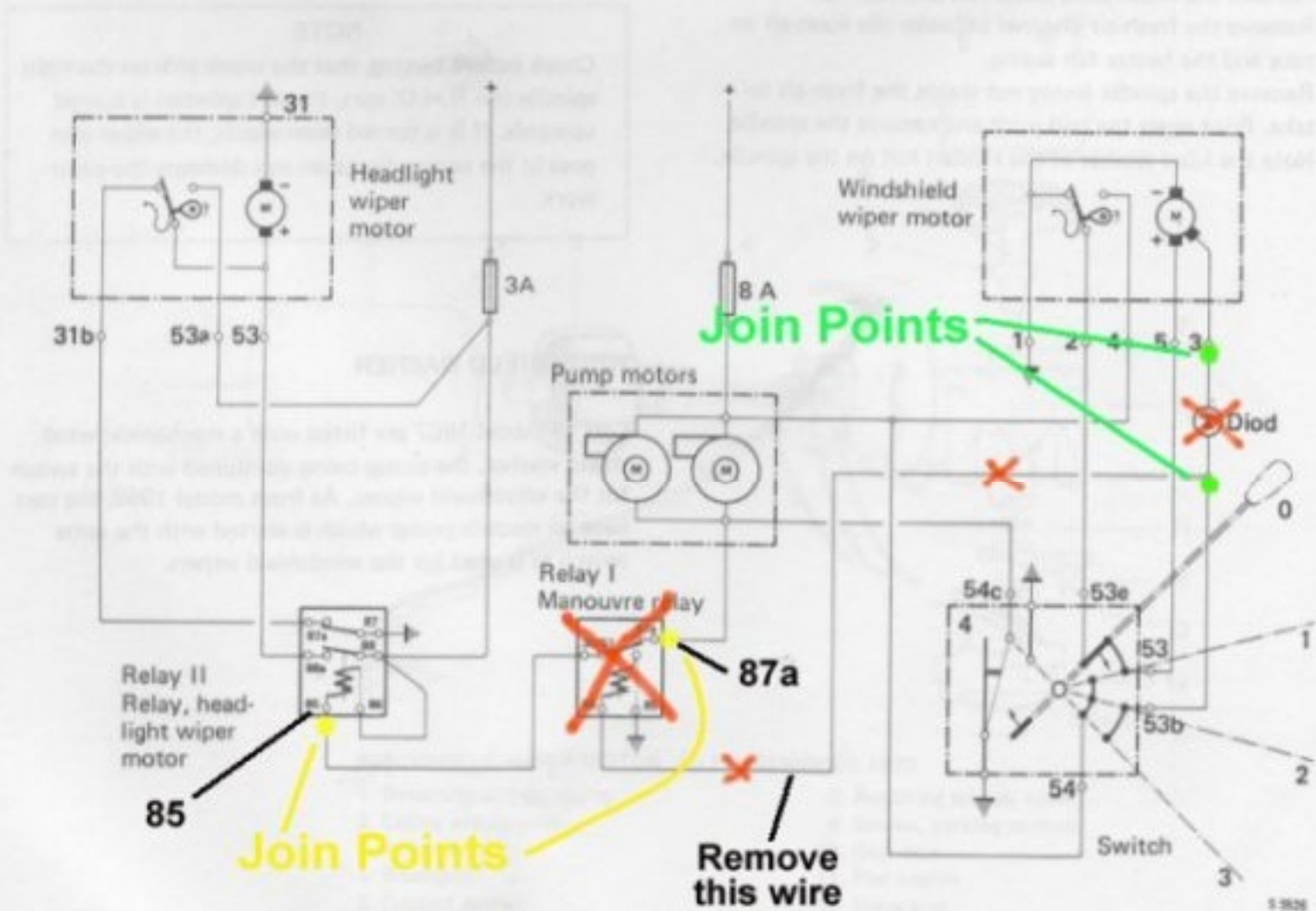
WIRING DIAGRAM, HEADLIGHT WIPERS AND WASHERS, MODEL 1971
